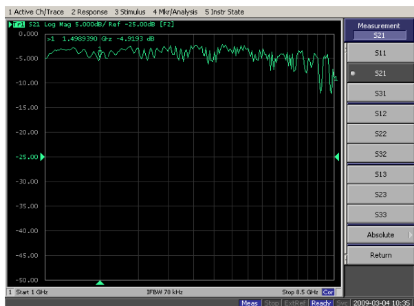
Figure 4: Insertion loss (S21) plot of 160 \mu\text{m} diameter RadWire, demonstrating broadband SW characteristic with 4 dB nominal loss.
