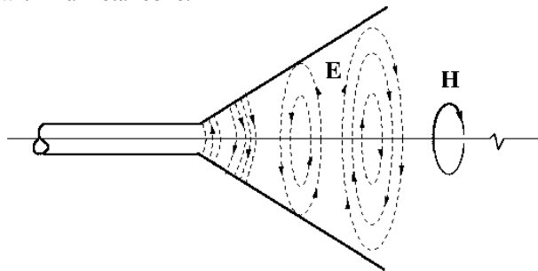
Figure 1: Surface wave evolution inside the launching cone.
