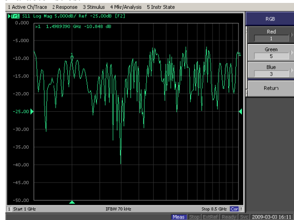
Figure 3: Return loss (S11) plot of 1.6 mm RadWire, showing nominal 10 dB or better (VSWR < 2:1), over 8 GHz.
