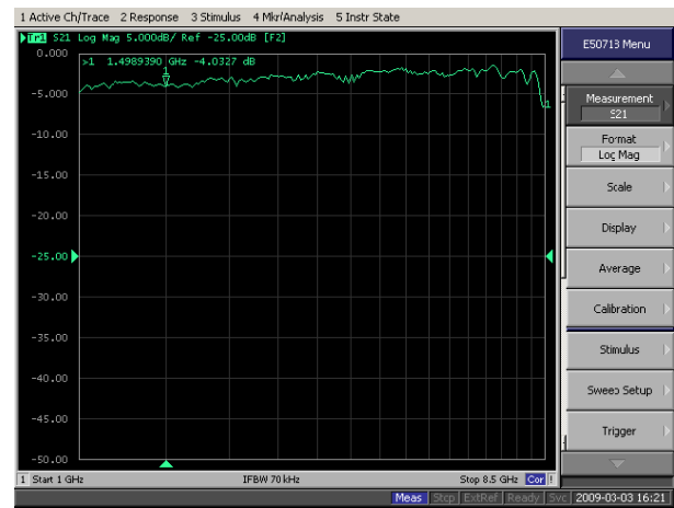
Figure 2: Insertion loss (S21) plot of 1.6 mm diameter RadWire, demonstrating broadband SW characteristic with 3-4 dB nominal loss.
